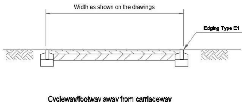
Figure 18 – Typical cycleway construction
